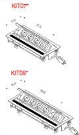
Single module in ABS for electricity and/or multimedia and system cable management. Colors available Anthracite RAL7016 and White RAL9010.
