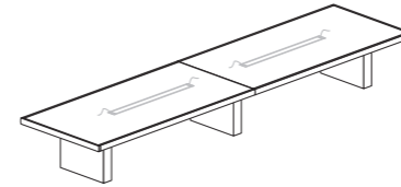
CX1635W+ELE L362 P122 H75 CX1647W+ELE L474 P122 H75
