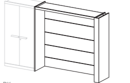
DX CXB119SD L177 P55,2 H202 CXB123SD L217 P55,2 H202
