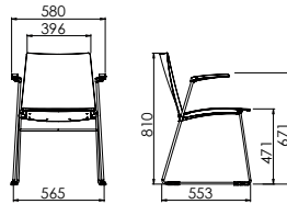
ARROW 410 SKID WITH ARMS
