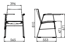
ARROW 410 SKID WITH WRITING TABLET
