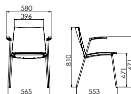
ARROW 410 4 LEG WITH ARMS
